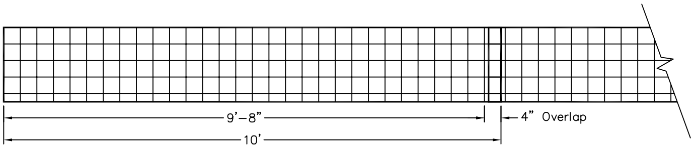
RIDGESCAPE FACING OVERLAP DETAIL
