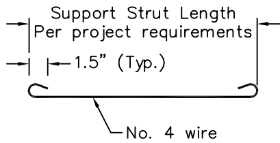
SUPPORT STRUT
