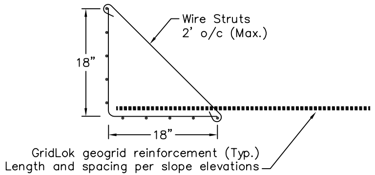
FACING CROSS SECTION
